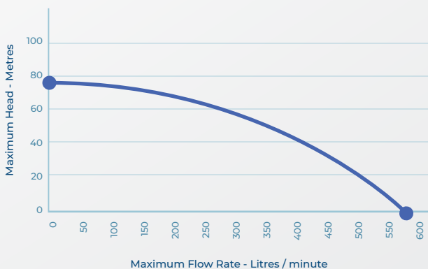
MH215-SHP PUMP PERFORMANCE CURVE
